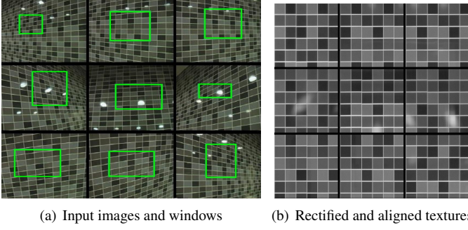
Figure 3. Camera calibration from images of an unknown pattern. The algorithm aligns the low-rank textures precisely despite specularities in the images. Although aligned and rectified, corresponding pixels do not have to correspond to the same 3D point.
